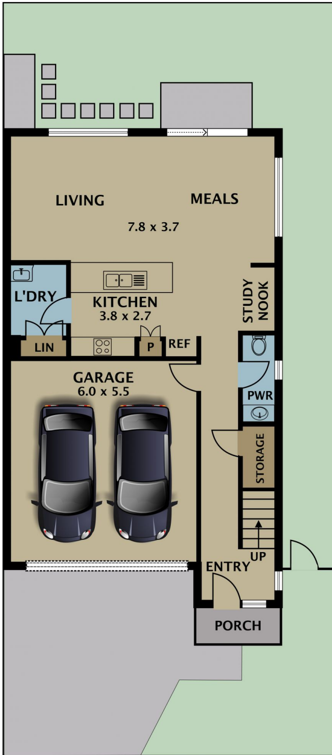
GROUND FLOOR
